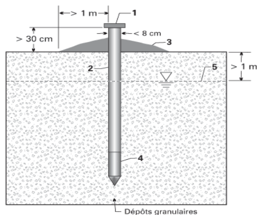
Figure 3 - Pointe filtrante
